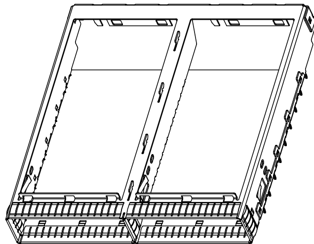
CAGE (1PCS)
