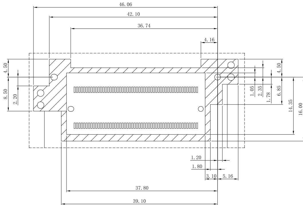
DETAIL B(2:1)
